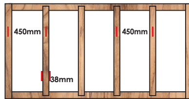
WOODEN FRAME TOP VIEW
